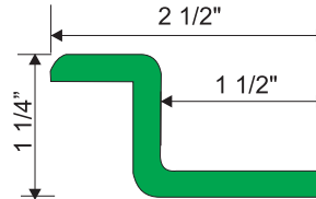
Z CLIPS .236 WALL X 2" WIDE
