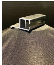
MP2B .090" WALL X 24' WITH 1" FLANGE STAPLE GROOVE OUT
