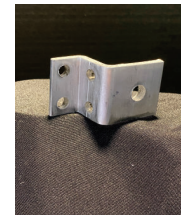
Z CLIPS .236 WALL X 2" WIDE
