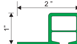
MP2A .090" WALL X 24' WITH 1" FLANGE STAPLE GROOVE DOWN
