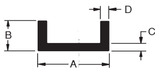
Channel
