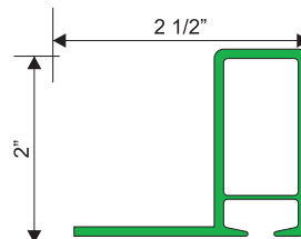
MP3A .090" WALL X 24" WITH 1 1/2" FLANGE STAPLE GROOVE DOWN
