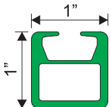
MP1A .090" WALL X 24' STAPLE GROOVE
