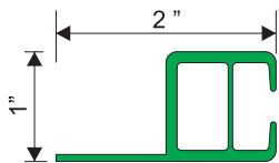
MP2B .090" WALL X 24' WITH 1" FLANGE STAPLE GROOVE OUT
