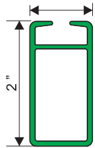
MP3 .090" WALL X 24" STANDARD STAPLE
