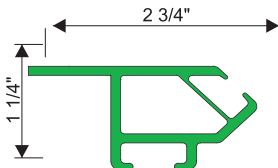
MP5B .090" WALL X 25' 6" SIGN FLEX RETAINER W/FLANGE STAPLE
