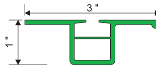
MP5 .090" WALL X 24" FASCIA BAND BLEED FRAME W/FLANGE STAPLE
