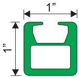
MP1 .125" WALL X 24' STAPLE GROOVE
