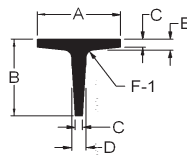
Tee / American Standard (Structural)
