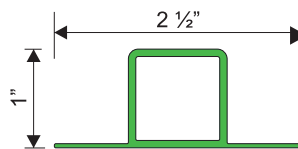
MI-56 .075" WALL X 24' WITH DOUBLE 3/4" FLANGES
