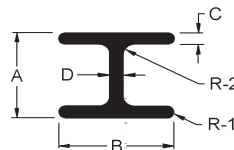
I Beam / American Standard (Structural)
