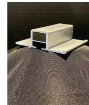
MP5 .090" WALL X 24" FASCIA BAND BLEED FRAME W/FLANGE STAPLE
