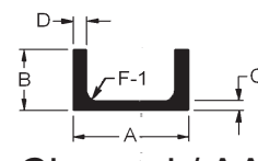
Channel / AA Aluminum Association
